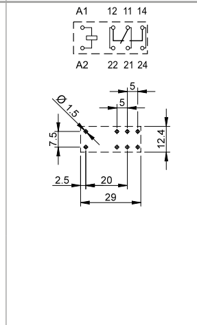
Copper side view Pin length 3.5 mm for PCB only Pin length 5.2 mm for PCB or sockets See ordering information
