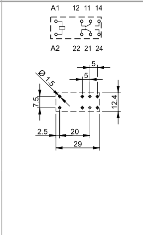
Copper side view Pin length 5.2 mm for PCB or sockets See ordering information
